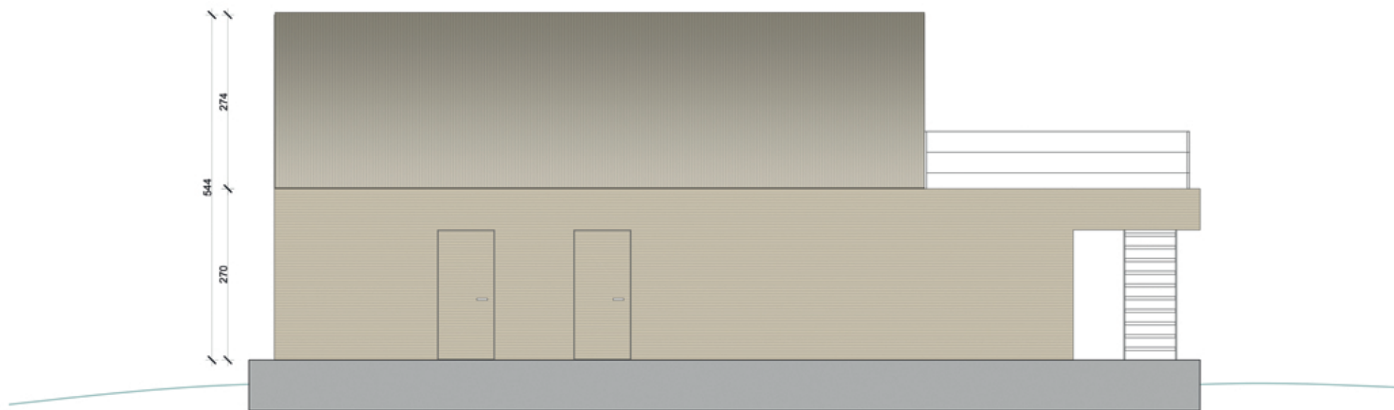
SIDE ELEVATION WITH THE ENTRANCE DOOR
