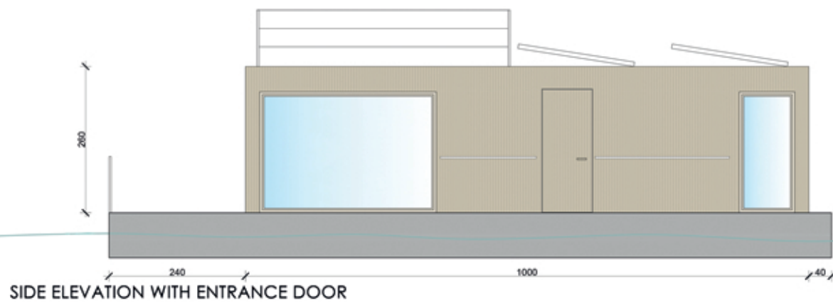
SIDE ELEVATION
